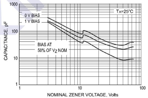
Fig.4 TYPICAL CAPACITANCE
